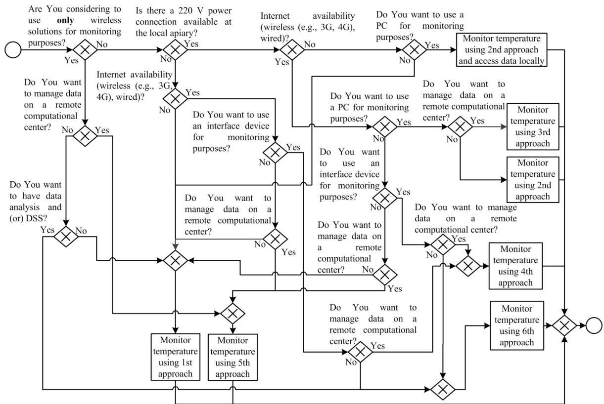
Fig. 8. Selection algorithm for system architectures.
