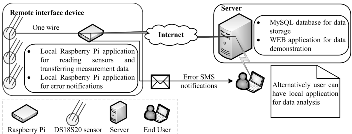
Fig. 4. System architecture with Raspberry Pi as an interface device.
