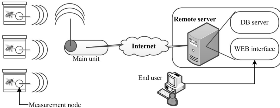
Fig. 6. Wireless measurement system used in ITAPIC project.
